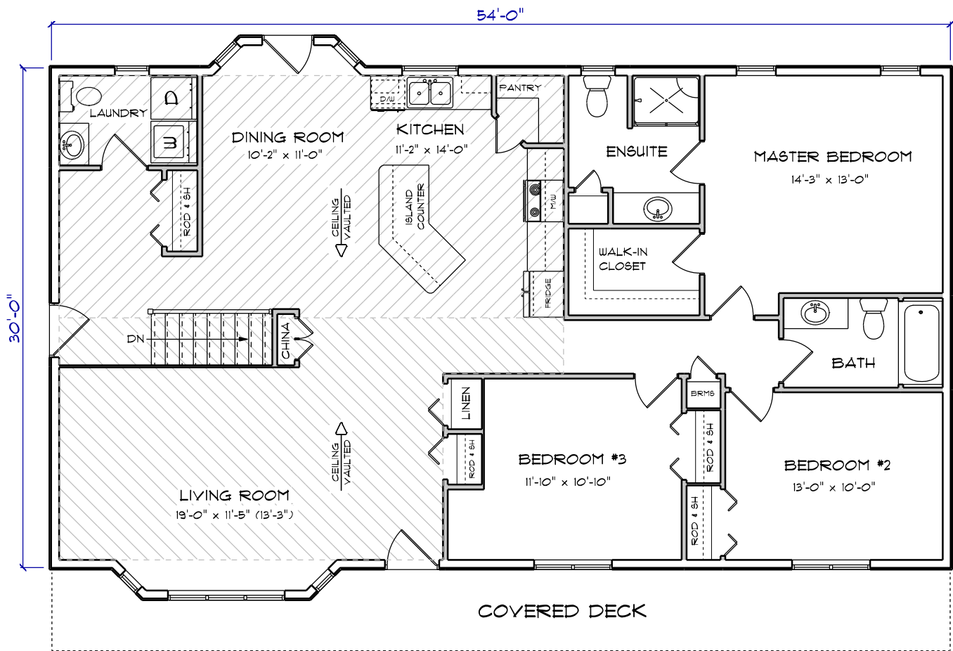
MAIN FLOOR PLAN 1651 SQ. FT.
