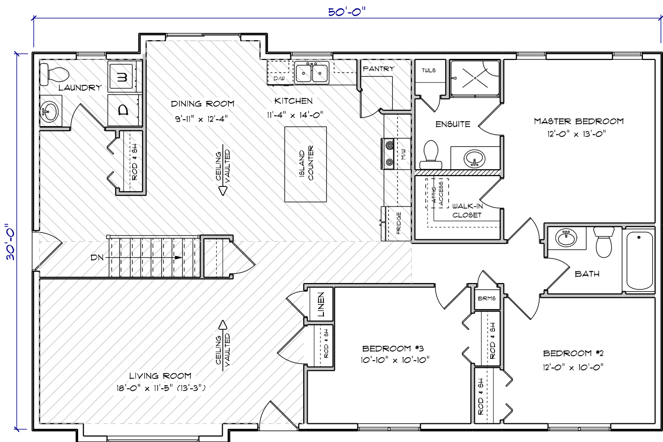
FLOOR PLAN
