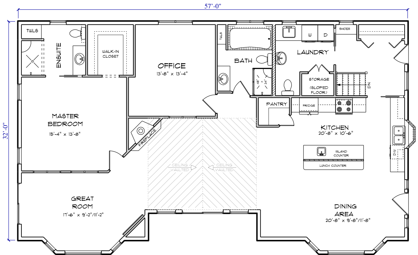
FLOOR PLAN
