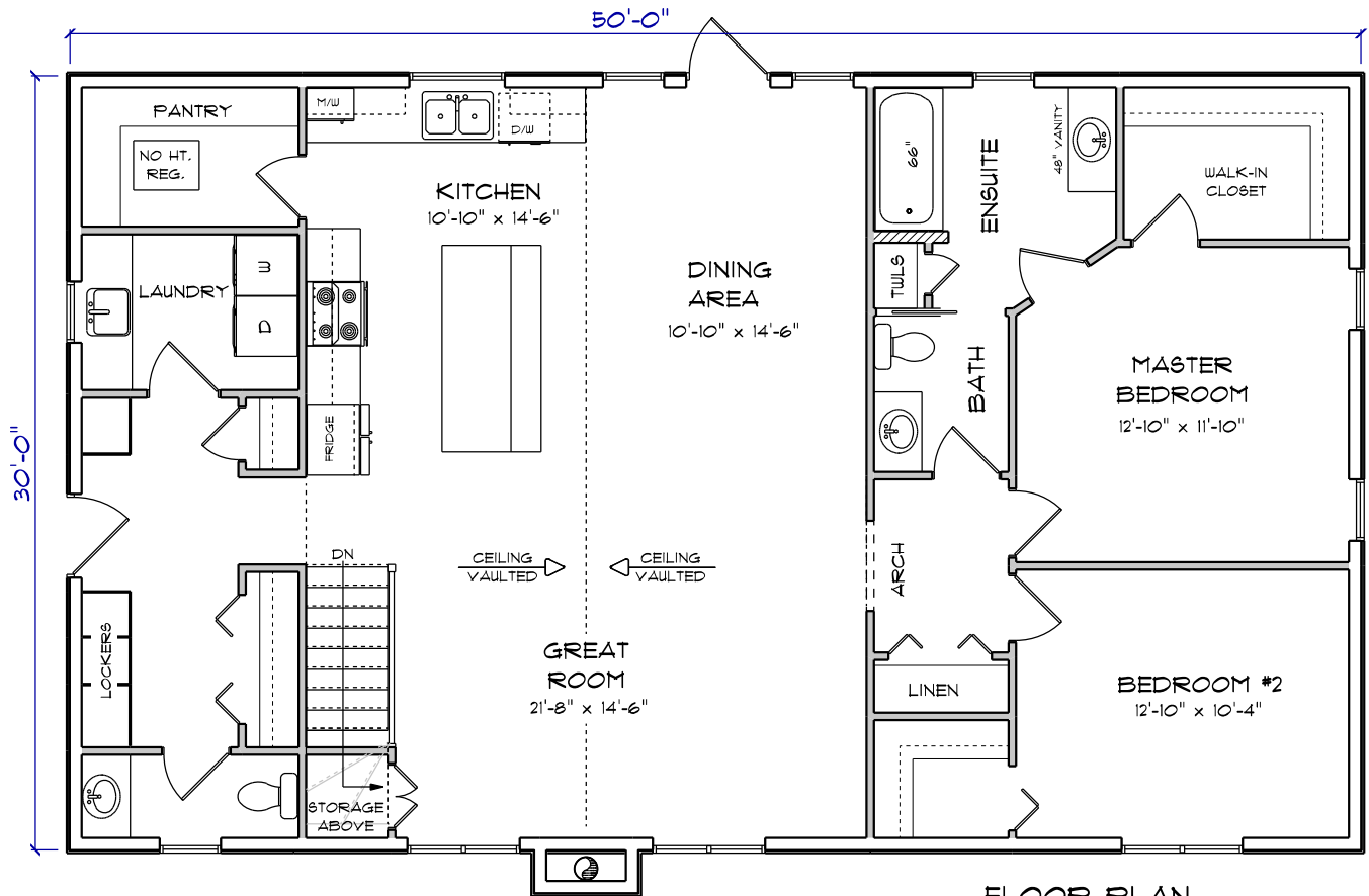
FLOOR PLAN
